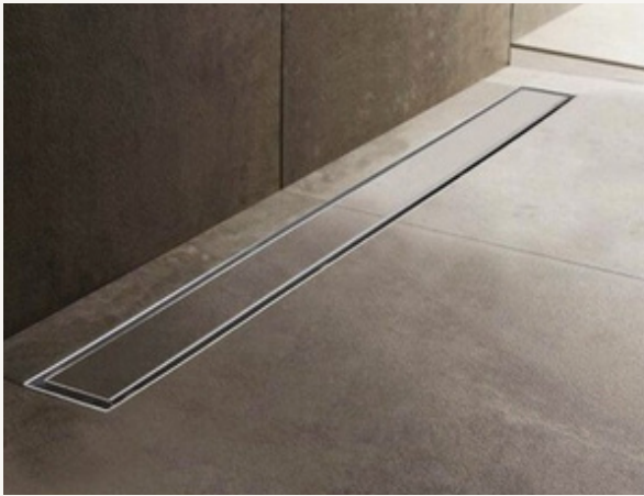
SHOWER DRAIN POINT ACO Shower Drain C 885 mm, with installation along the wall and tiled decorative cover, stainless steel
